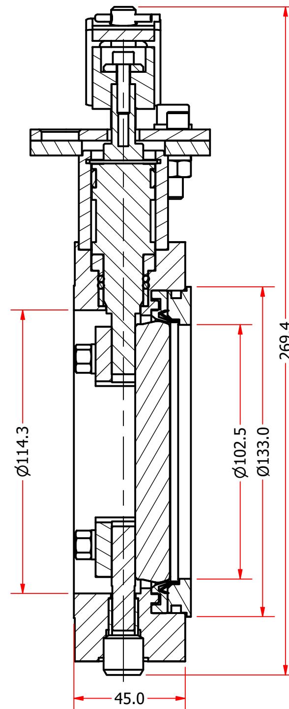
SECTION A-A SCALE 1 / 1.5
