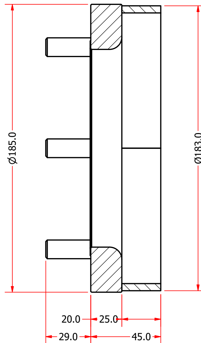
SECTION A-A SCALE 1 / 1.5
