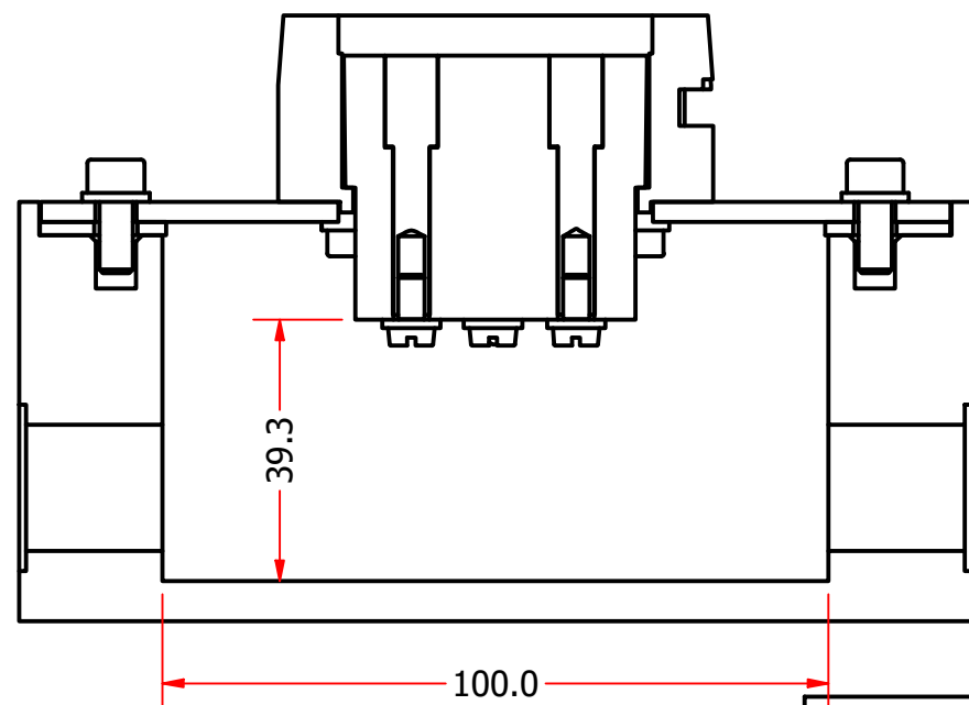
SECTION A-A SCALE 1 / 1.25
