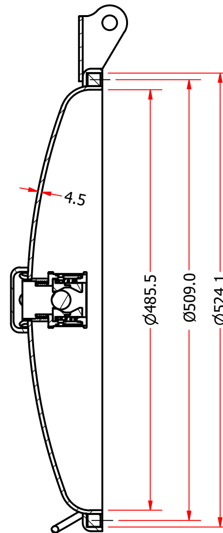
SECTION A-A SCALE 1 / 4.25
