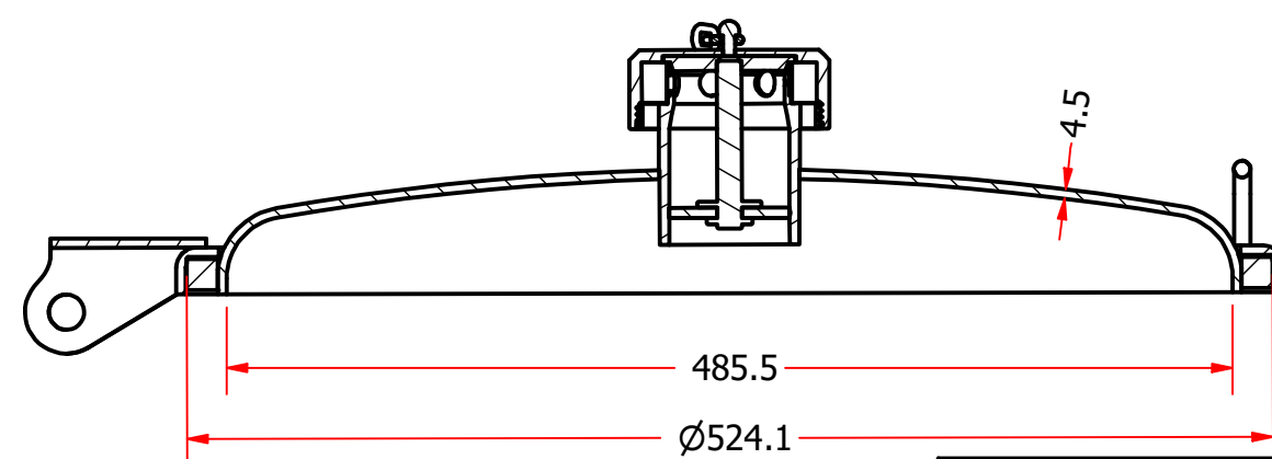
SECTION A-A SCALE 1 / 4
