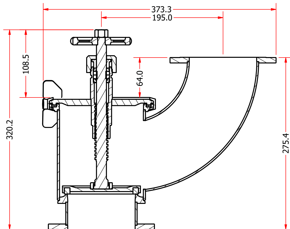
SECTION A-A SCALE 1 / 3.1
